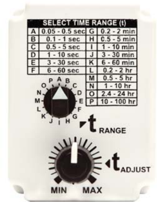
Select one of 16 Time Ranges with rotary switch
