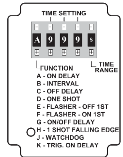
Figure 1- Multi-Function (TD-781)
